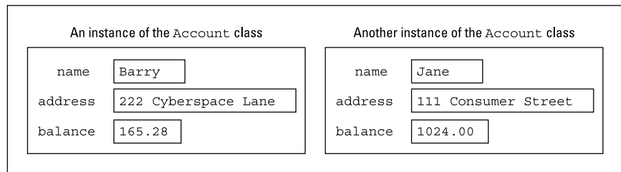
FIGURE 7-1: Two objects.
