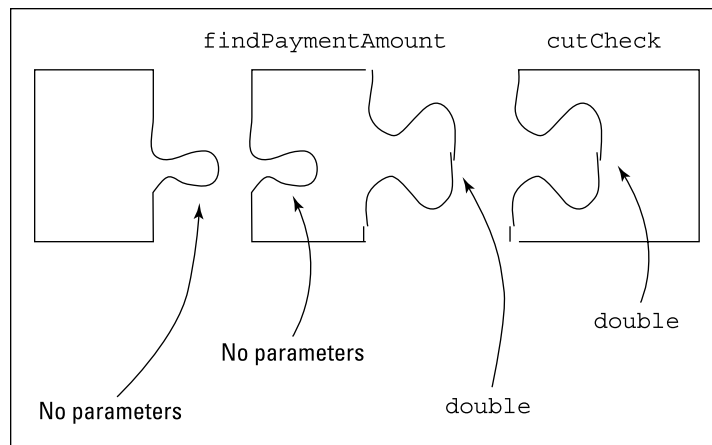
FIGURE 8-7: Matching parameters.
