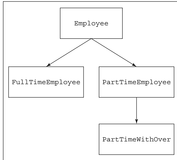
FIGURE 8-8: A tree of classes.
