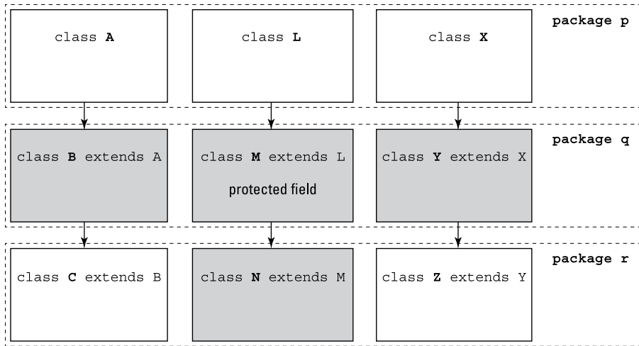
FIGURE 14-9: The range of code in which a protected field or method can be used (shaded).
