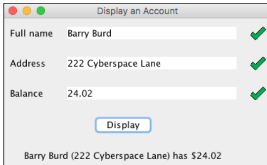
FIGURE 7-20: I'm rich.
