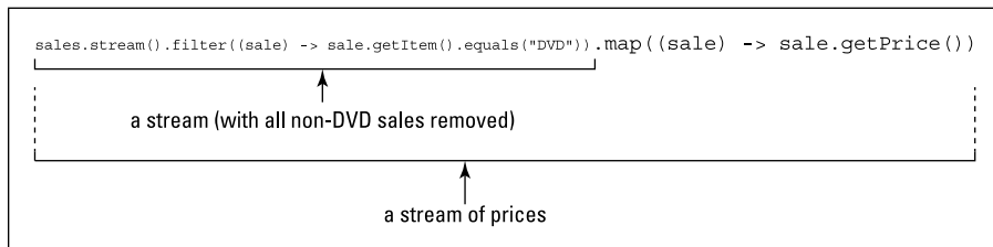
FIGURE 12-13: Getting the price from each DVD sale.
