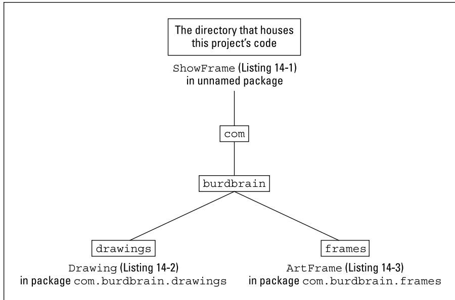
FIGURE 14-5: The files and directories in your project.
