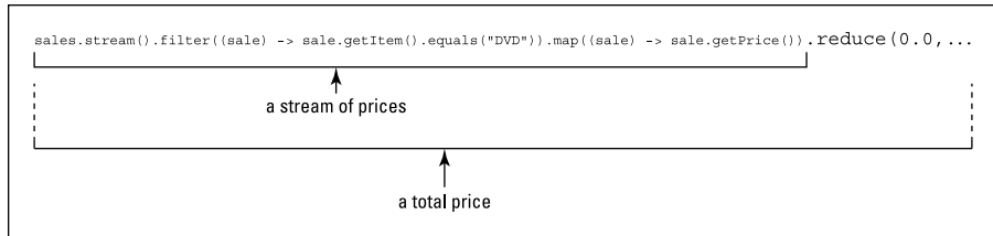
FIGURE 12-14: Getting the total price of all DVD sales.
