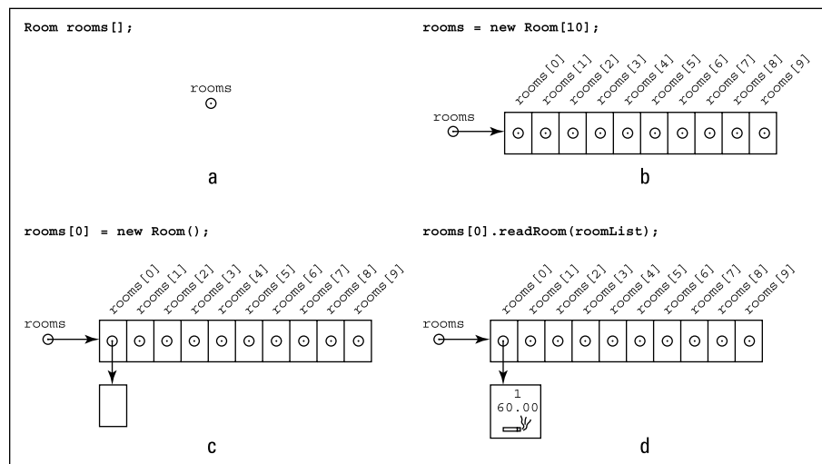
FIGURE 11-11: Steps in creating an array of objects.
