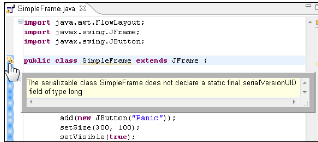
FIGURE 9-4: Without a Suppress Warnings annotation, Java warns you about a missing serialVersion UID field.
