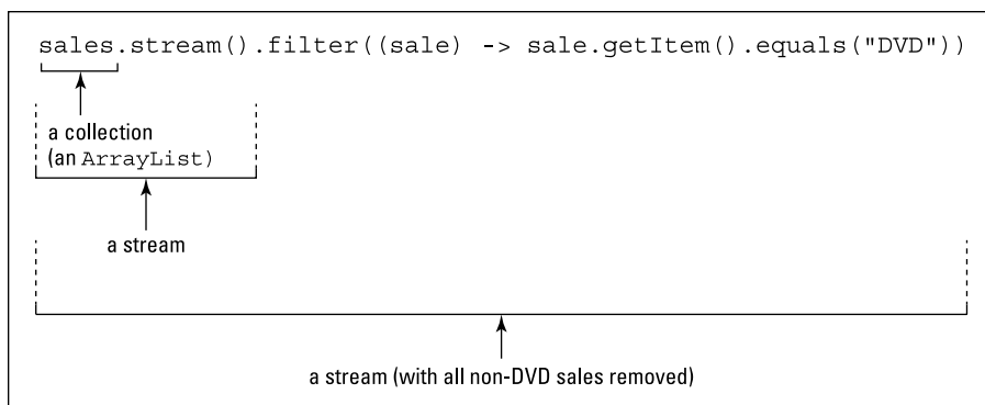
FIGURE 12-12: Getting all DVD sales.
