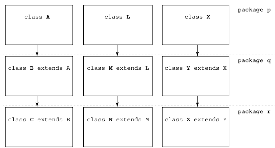
FIGURE 14-7: Packages cut across subclass hierarchies.
