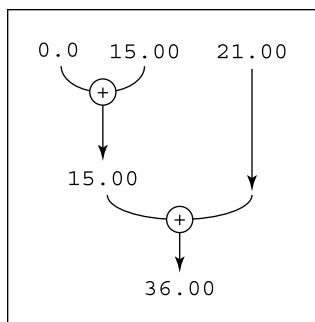
FIGURE 12-10: The reduce method adds two values from an incoming stream.
