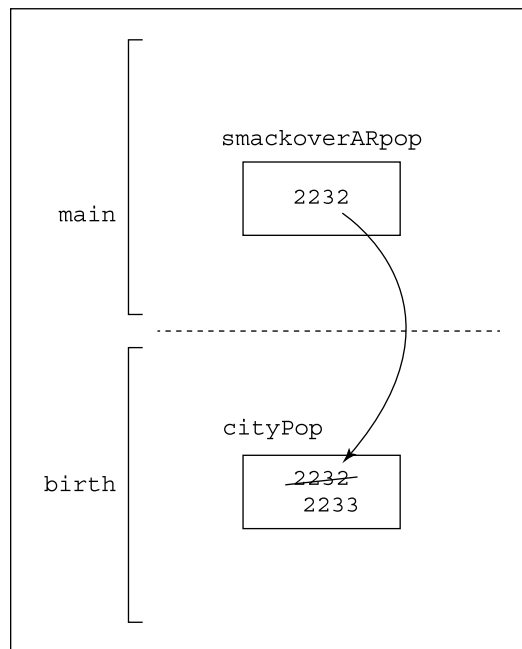
FIGURE 10-11: Pass by value, under the hood.
