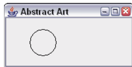
FIGURE 14-4: An ArtFrame .
