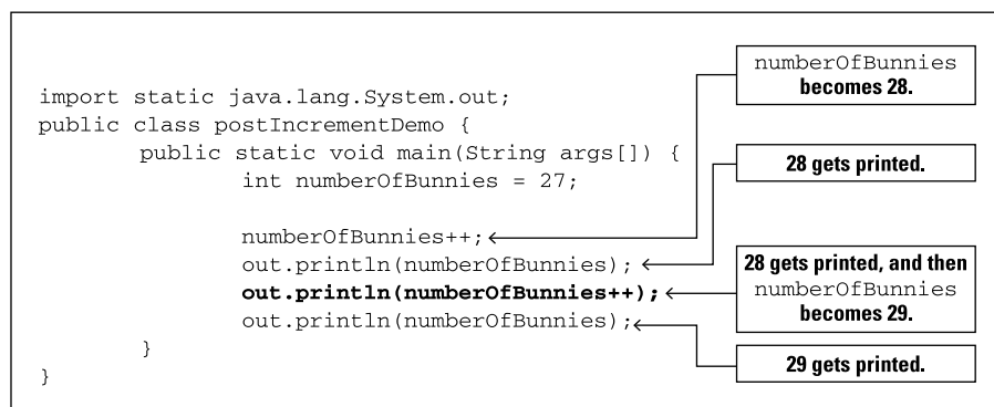
FIGURE 4-15: Using postincrement.
