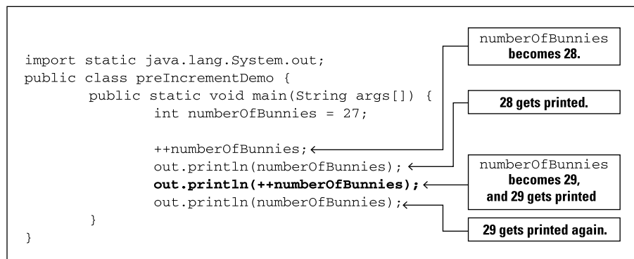
FIGURE 4-13: Using preincrement.
