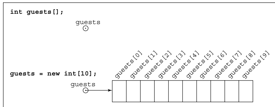
FIGURE 11-2: Two steps in creating an array.
