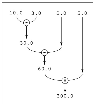
FIGURE 12-11: The reduce method multiplies values from an incoming stream.
