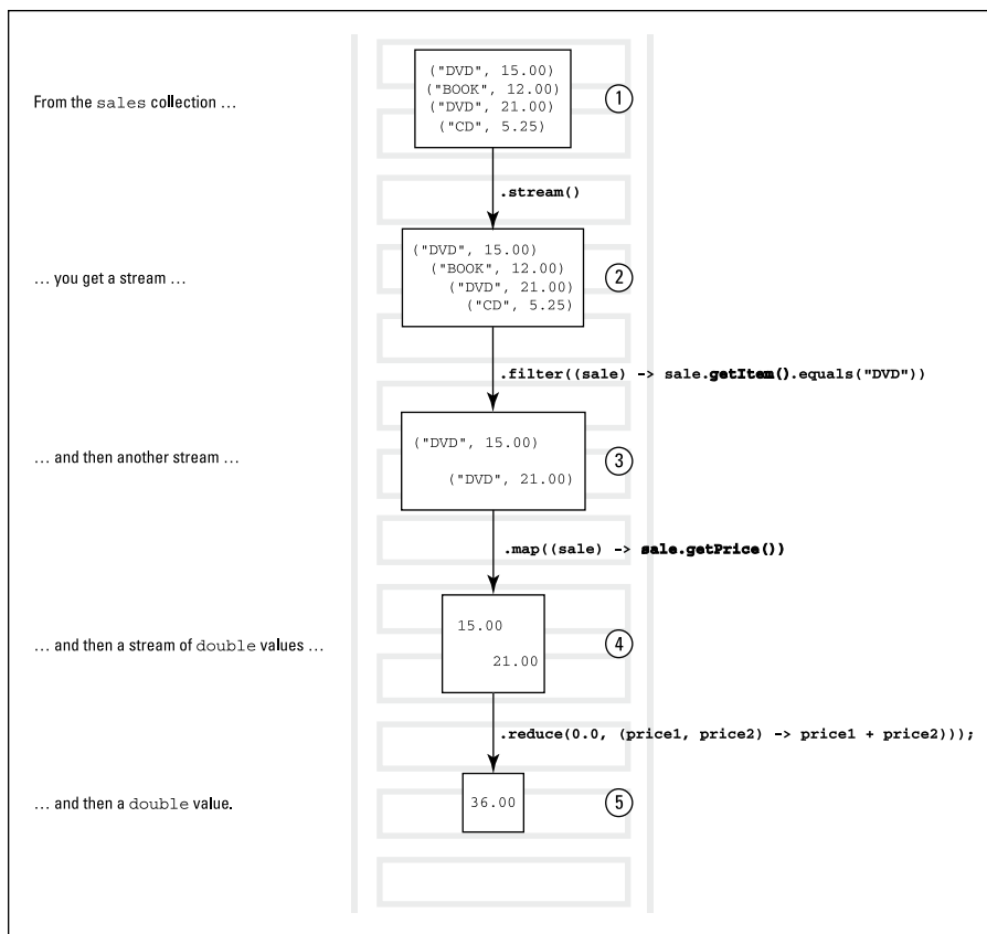
FIGURE 12-9: A functional programming assembly line.
